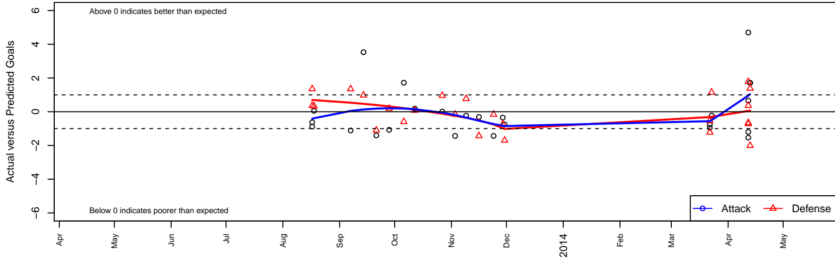
West Coast FC United B96 Dots are actual minus expected GF (blue circles) and GA (red triangles). Blue line is smoothed change in attack strength. Red is smoothed change in defense strength.
